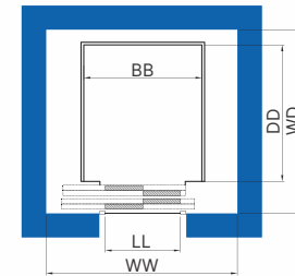
Single entrance car Side opening
