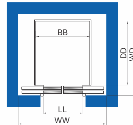
Single entrance car Centre opening
